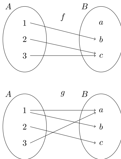
Figure 1.6: Mappings and relations
