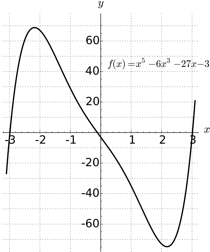
Figure 23.31: The graph of f(x) = x^5 - 6x^3 - 27x - 3
