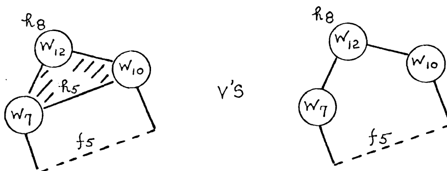
Fig. 13. Illustrations for Example 4.
