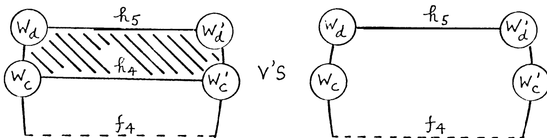
Fig. 10c. To find f_4
