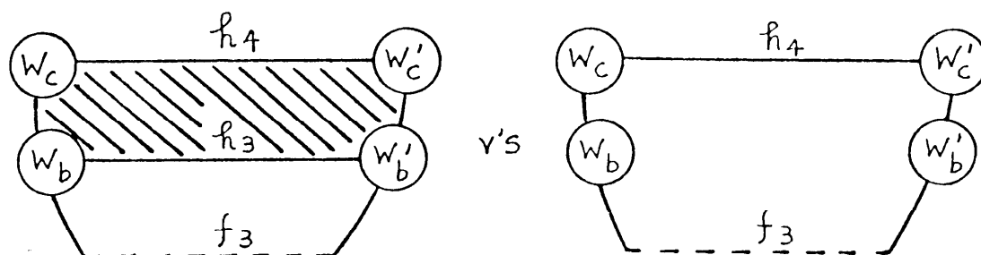
Fig. 9g. To find f_3 .
