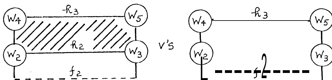
Fig. 13g. To find f_2 .
