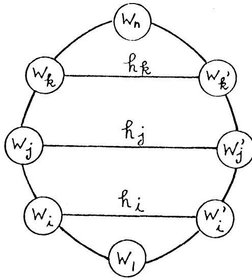
Fig. 6. An octagon with three potential h-arcs.
